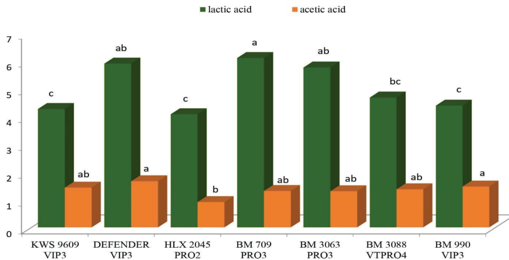
Figure 3. Percentage of lactic acid and acetic acid in silage produced from different maize hybrids. *Means followed by the same letters on the bars do not differ by Tukey's test at 5% probability.
